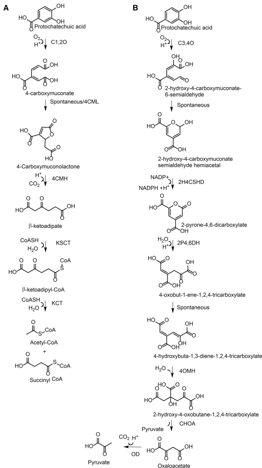
Figure 1. Microbial pathways for the catabolism of aromatic compounds using protocatechuic acid. Ortho -ring cleavage (intradiol cleavage) by catechol-1,2-dioxygenase (C1,2O; A) or meta -cleavage (extradiol cleavage) by catechol-3,4-dioxygenase (C3,4O; B) determines the catabolic fate of the ring-opened product. 4CML, 4-Carboxymuconate lactonase; 4CMH, 4-carboxymuconolactone hydrolase; KSCT, \beta -ketoadipate:succinyl-CoA transferase; KCT, \beta -ketoadipyl-CoA thiolase; 2H4CSHD, 2-hydroxy-4-carboxymuconate-6-semialdehyde dehydrogenase; 2P4,6DH, 2-pyrone-4,6-dicarboxylate hydrolase; 4OMH, 4-oxalomesaconate hydratase; CHOAs, 4-carboxy-4-hydroxy-2-oxoadipate aldolase; OD, oxaloacetate \beta -decarboxylase.
